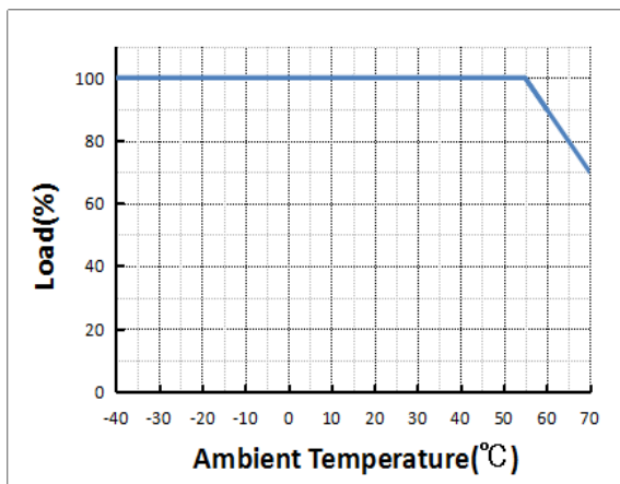
Output Power-Temperature
