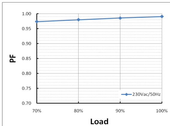
▲ Power Factor
