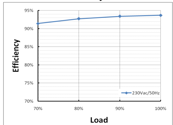
▲ Efficiency
