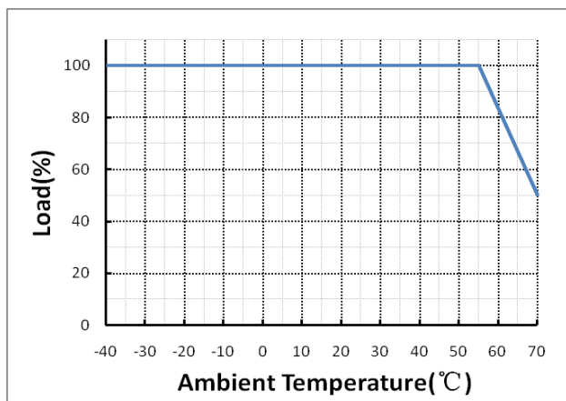
Output Power-Temperature
