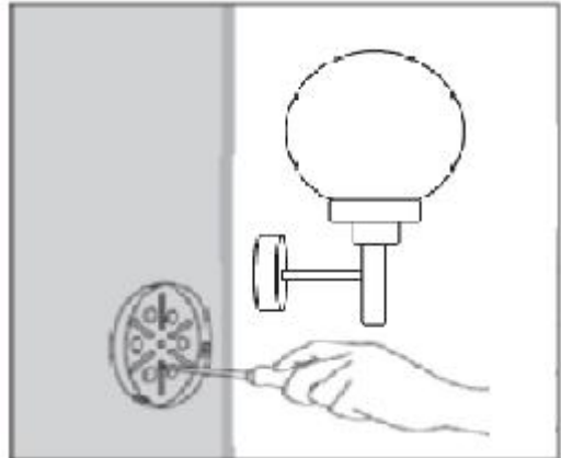
2.) Put on the lighting to mounting bracket fixed with screw
